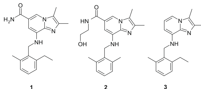
Figure 1. Examples of imidazo[1,2- a ]pyridine APAs.
